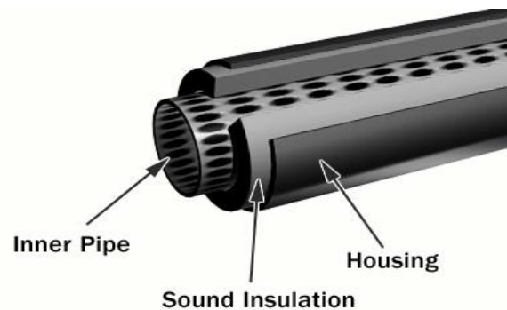
Fig. 3.2 Absorptive automotive muffler
