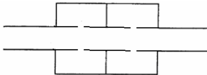
Fig. 3.11 Resonating chamber muffler
