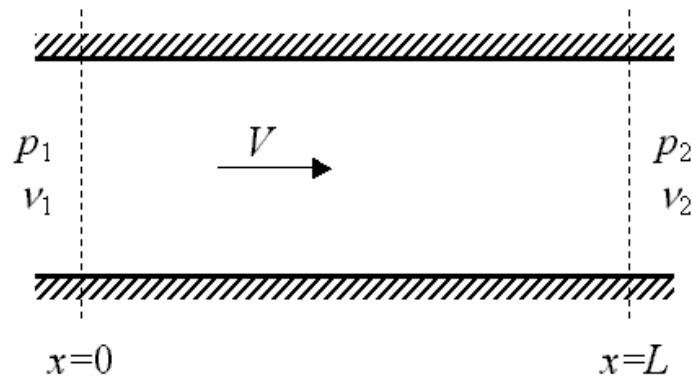
Fig.4.1. Plane wave propagation in a rigid straight pipe transporting a turbulent incompressible mean flow
