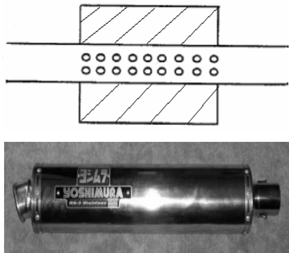
Fig. 3.7 Straight through absorption muffler
