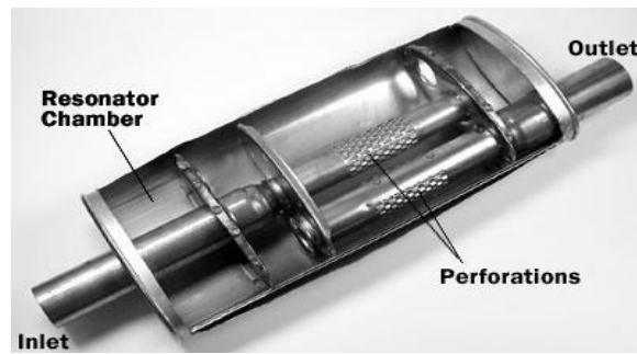
Fig. 3.1 Reactive automotive muffler
