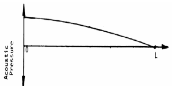
Fig. 3.3 Quarter wavelength
