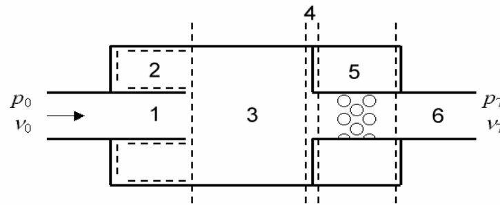
Fig.4.2 Real muffler
