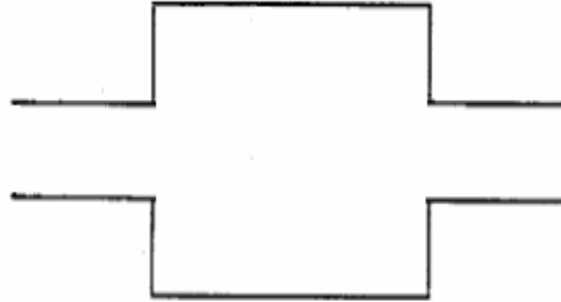
Fig. 3.4 Simple Expansion Chamber
